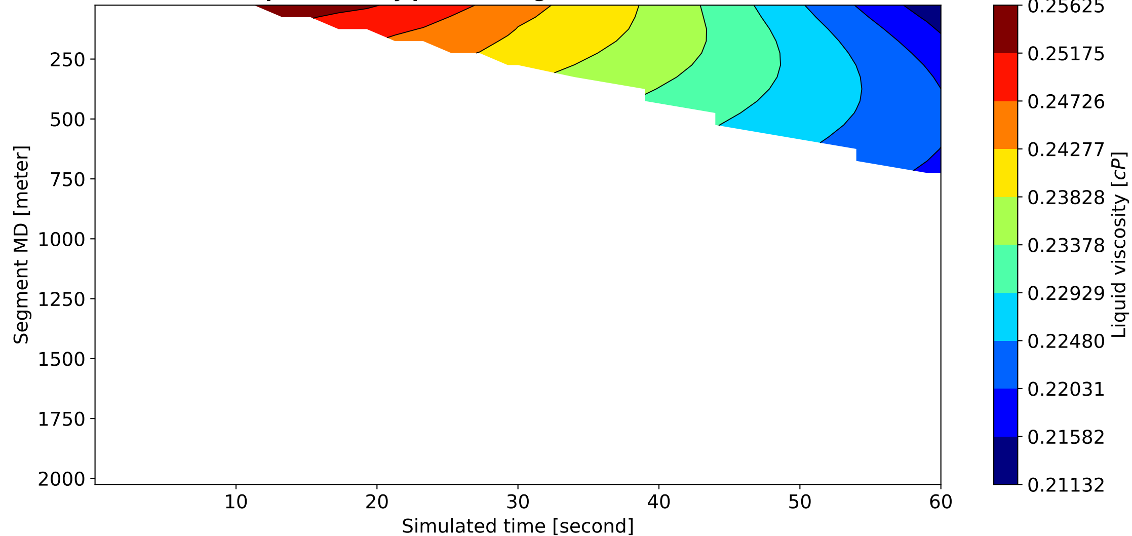
Liquid viscosity profile along the wellbore over time
